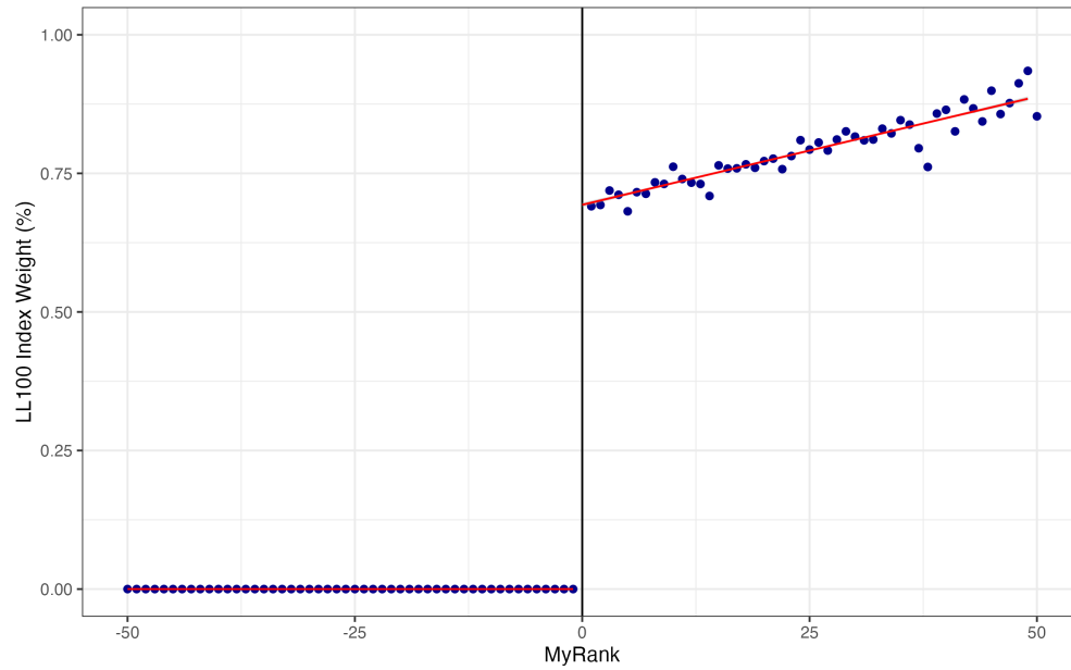
Figure 1: LSTA 100 Index
